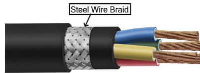
Steel Wire Braid Armoured Cable
